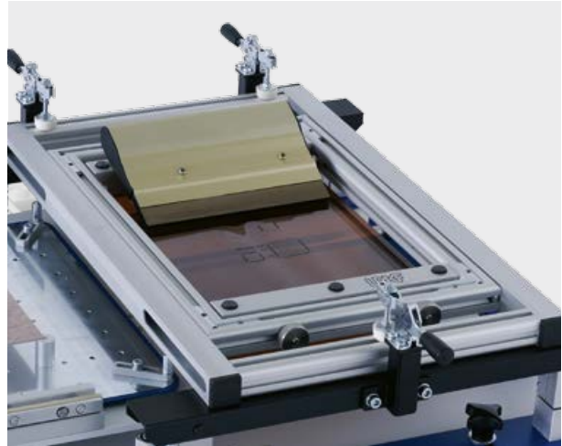
LPKF ProtoPrint S with a polyimide stencil. Metal stencils can be used as well (cover picture).
