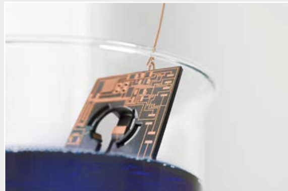
4. Selective metallization with LPKF ProtoPlate
